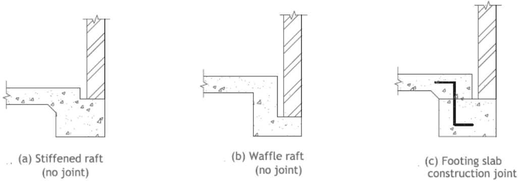
Figure* 1: Footing systems requiring joint treatments
